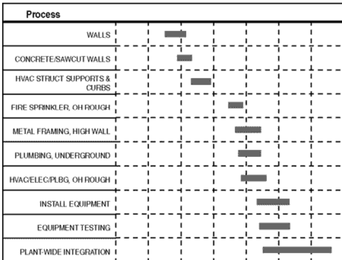
Gantt Chart.
